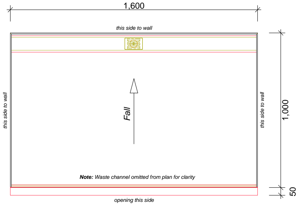
Floor Plan Chicago - Linea Quattro Channel Drain & Stainless Steel Cover 1600x1000 3WChiBack_1600x1000
