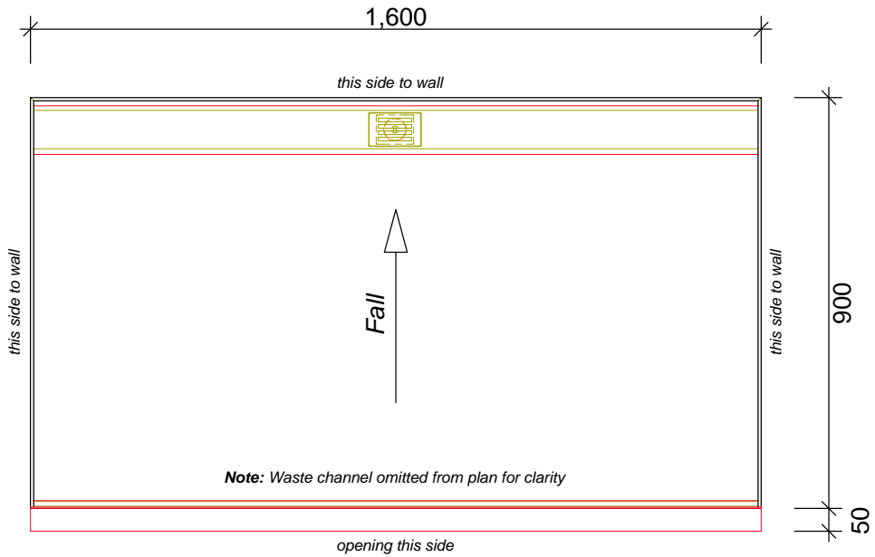
Floor Plan Ottawa - Linea Quattro Channel Drain & Stainless Steel Cover 1600x900 3WOttBack_1600x900
