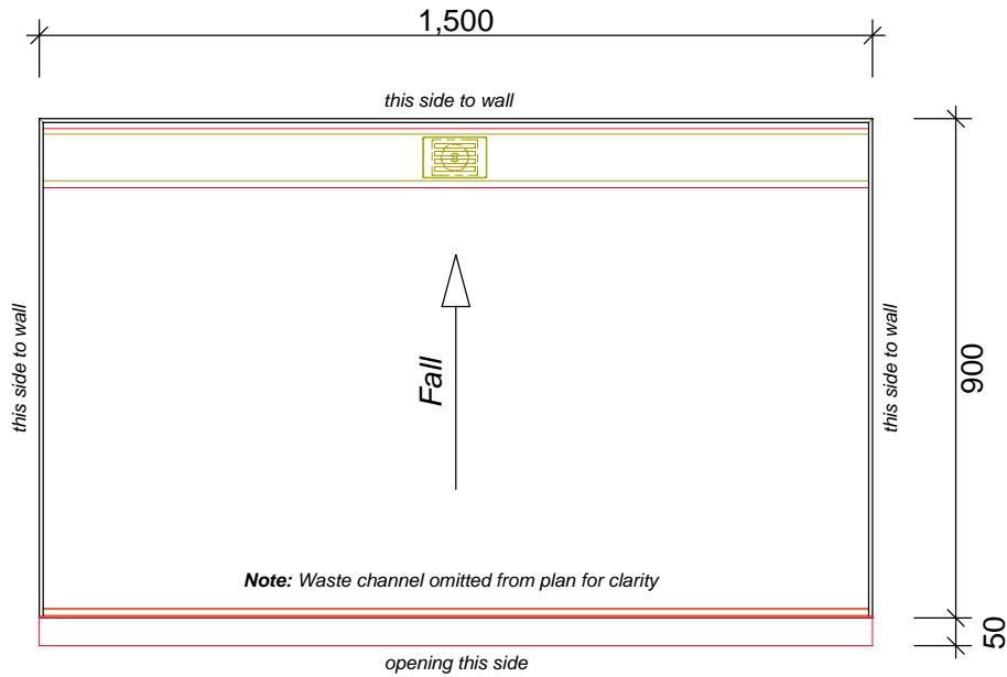
Floor Plan Barcelona - Linea Quattro Channel Drain & Stainless Steel Cover 1500x900 3WBarBack_1500x900
