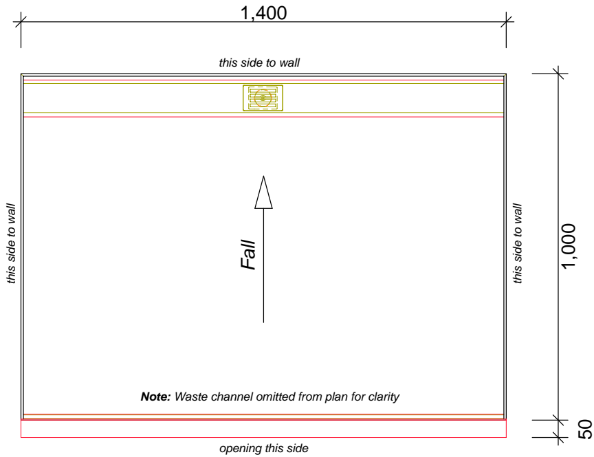
Floor Plan Lisbon - Linea Quattro Channel Drain & Stainless Steel Cover 1400x1000 3WLisBack_1400x1000
