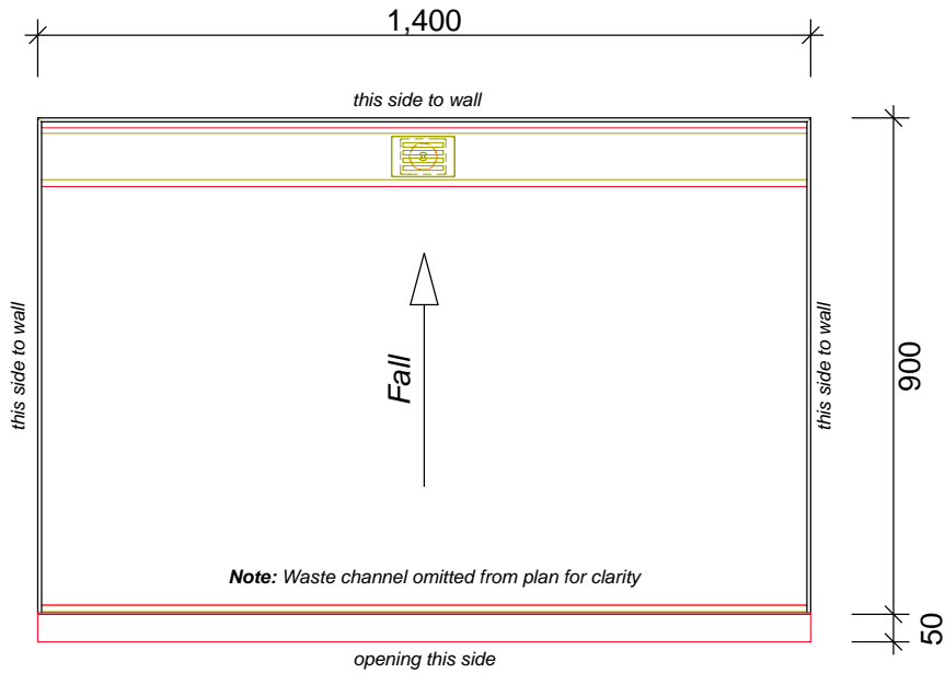
Floor Plan Santiago - Linea Quattro Channel Drain & Stainless Steel Cover 1400x900 3WSanBack_1400x900
