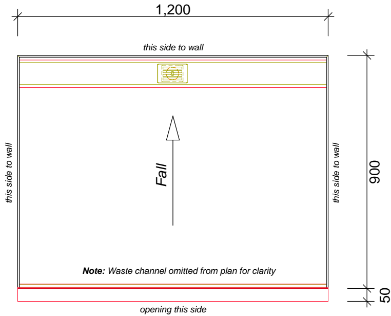
Floor Plan Berlin - Linea Quattro Channel Drain & Stainless Steel Cover 1200x900 3WBerBack_1200x900
