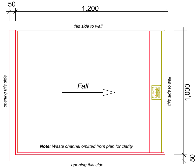
Floor Plan Shanghai - Linea Quattro Channel Drain & Stainless Steel Cover 1200x1000 2WShaRH_1200x1000
