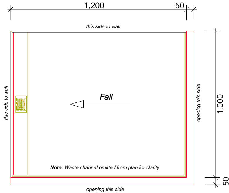
Floor Plan Shanghai - Linea Quattro Channel Drain & Stainless Steel Cover 1200x1000 2WShaLH_1200x1000
