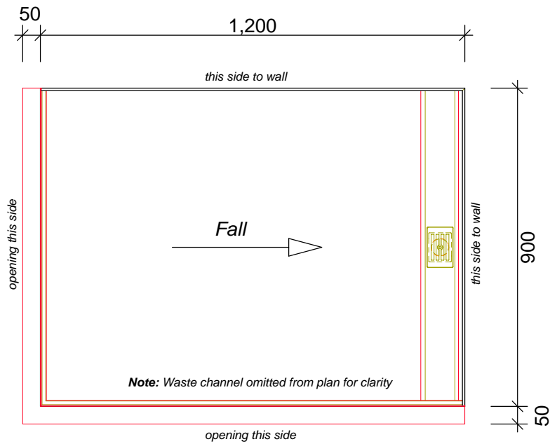
Floor Plan Milan - Linea Quattro Channel Drain & Stainless Steel Cover 1200x900 2WMiIRH_1200x900
