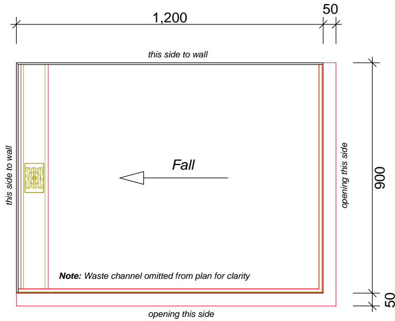
Floor Plan Milan - Linea Quattro Channel Drain & Stainless Steel Cover 1200x900 2WMiLH_1200x900
