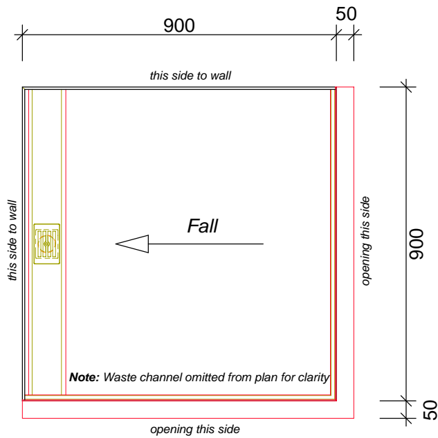
Floor Plan Dublin - Linea Quattro Channel Drain & Stainless Steel Cover 900x900 2WDubLH_900x900
