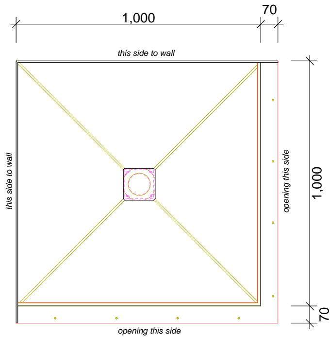
Floor Plan Sensation - Cuub centred tile-over waste 1000x1000 2WSens_1000x1000
