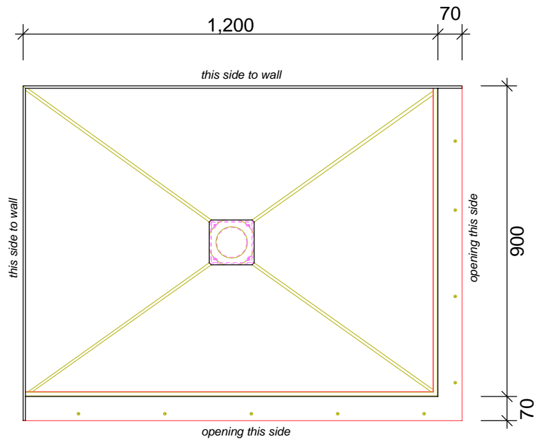
Floor Plan Bella - Cuub centred tile-over waste 1200x900LH 2WBell_1200x900LH
